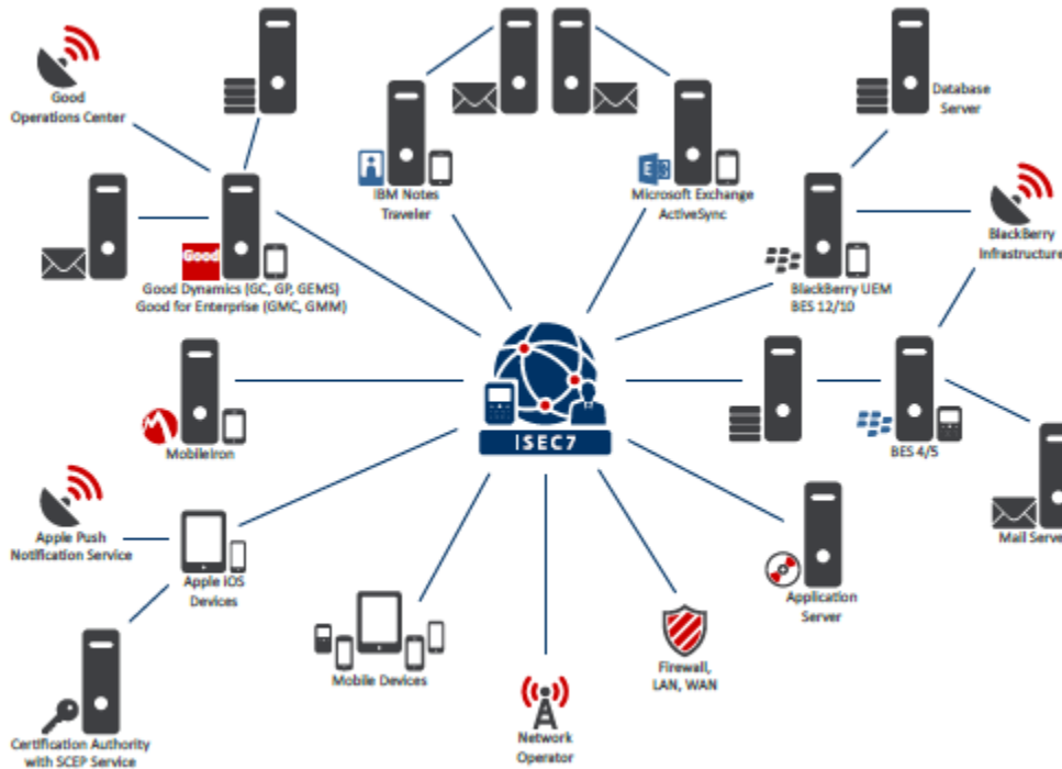
Figure 1-1: ISEC7 EMM Suite Architecture
