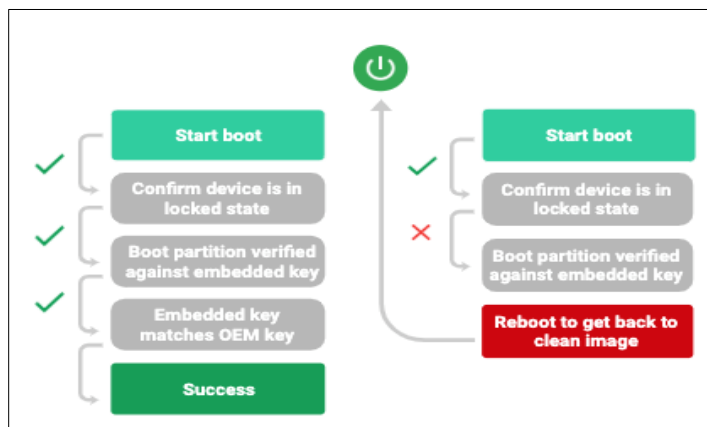
Figure 2-2: Verified Boot
