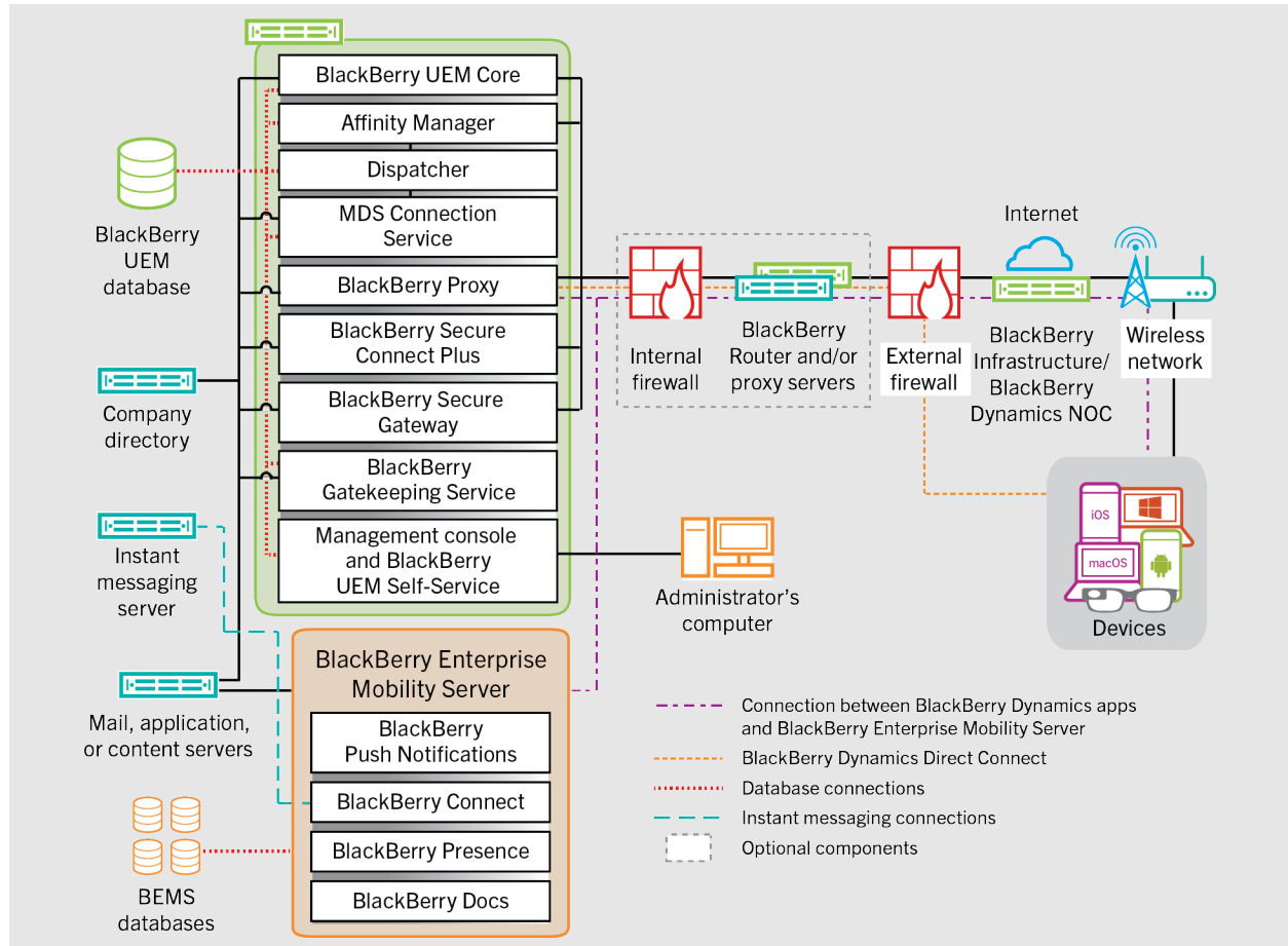
Figure 2-1: BEMS/UEM Architecture
