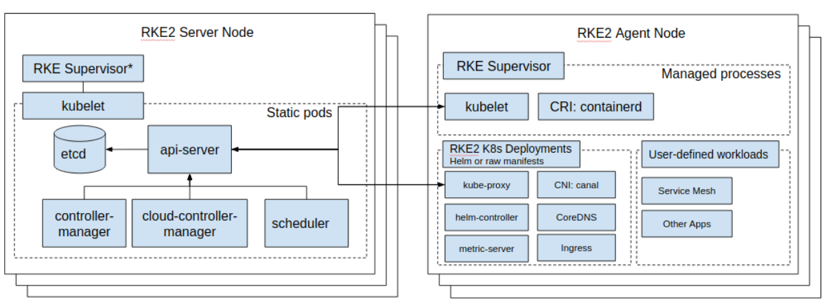
Figure 2-1: RKE2 Architecture
